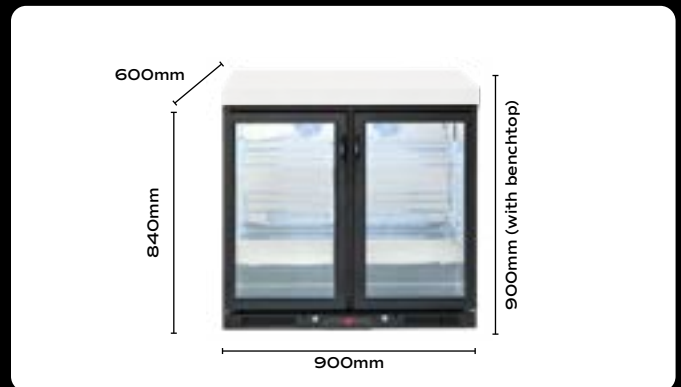
Double fridge FRIDGE-DDBLK - 208L, black double door fridge only (flat benchtop to suit is additional).
